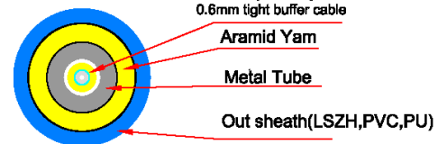
3, Cable Profile View
